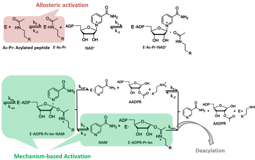
Fig. 1. Chemical mechanism of sirtuin-catalyzed deacylation and modes of sirtuin activation. Following sequential binding of acylated peptide substrate and \text{NAD}^+ cofactor, the reaction proceeds in two consecutive stages: i) cleavage of the nicotinamide moiety of \text{NAD}^+ (ADP-ribosyl transfer) through the nucleophilic attack of the acetyl-Lys side chain of the protein substrate to form a positively charged O-alkylimidate intermediate (depicted above), and ii) subsequent formation of deacylated peptide. For simplicity, all steps of stage ii as well as \text{AADPR} + \text{Pr} dissociation are depicted to occur together with rate limiting constant k_{\text{cat}} . Red: Allosteric activation increases the affinity of a limited set of peptide substrates for the SIRT1 enzyme only and requires an allosteric binding site. Green: Mechanism-based activation is a new mode of enzyme activation that relies on the conserved sirtuin reaction mechanism rather than an increase in the affinity of selected peptide substrates.
