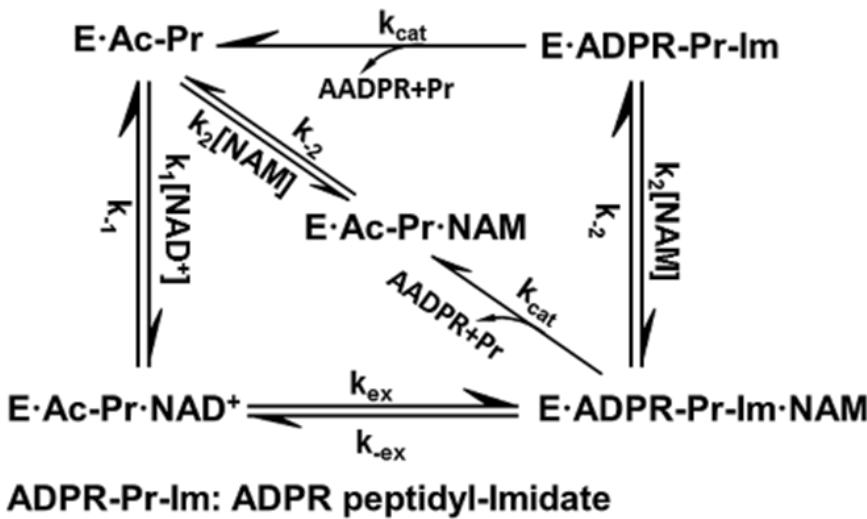
Fig. 2. General model for sirtuin-catalyzed deacylation in the presence of \text{NAD}^+ and NAM. This model, based on the reaction mechanism depicted in Fig. 1, provides a minimal kinetic model that captures the essential features of sirtuin deacylation kinetics suitable for predicting the effects of mechanism-based modulators on sirtuin activity. In the presence of saturating Ac-Pr, E is rapidly converted into E·Ac-Pr and NAM binding to E can be neglected, resulting in a simplified reaction network with 5 species. Ac-Pr, acetylated peptide; ADPR, adenosine diphosphate ribose; AADPR, O-acetyl adenosine diphosphate ribose.
