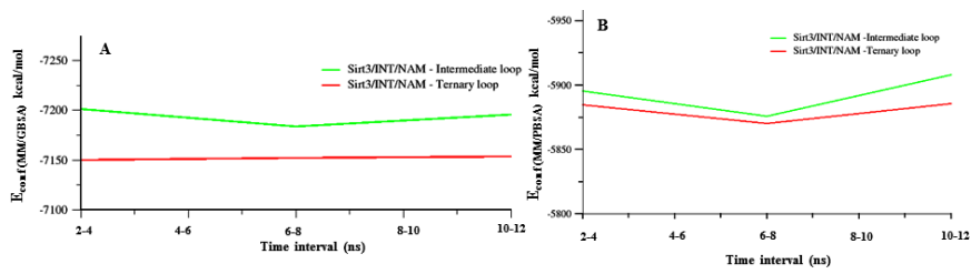
Fig. 7. Conformational energies of Sirt3-Int-NAM complexes. Conformational energies estimated using MM/PBSA and MM/GBSA method showing the energy gap for the Sirt3/INT/NAM complexes with different cofactor loop conformation. SIRT3/INT/NAM prepared from 4FVT with loop residues (res 155-178) replaced from 4BVG is shown in green and SIRT3/INT/NAM prepared from 4FVT with its native loop is shown in red. Panel A shows a plot of MM/GBSA conformational energy vs time and B shows plot of MM/PBSA vs times for the two different conformers.
